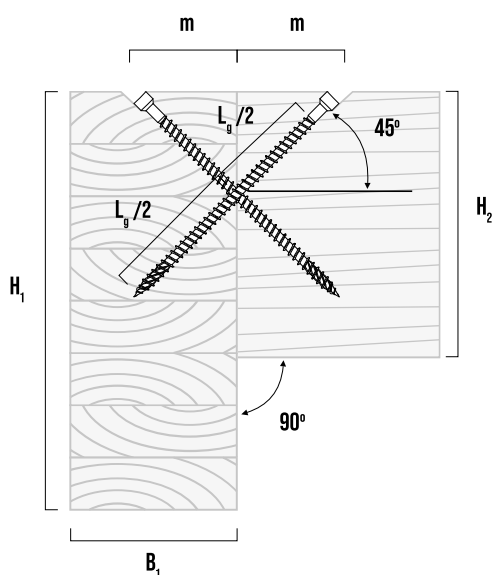
Cross-section
