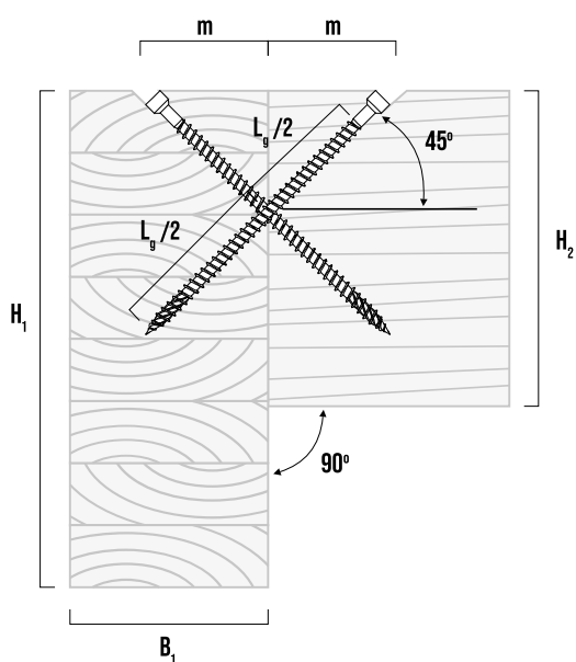
Cross-section
